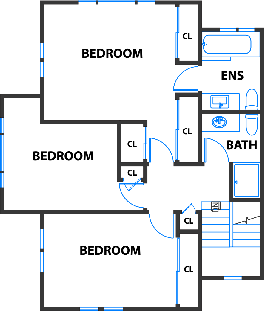
SECOND FLOOR
